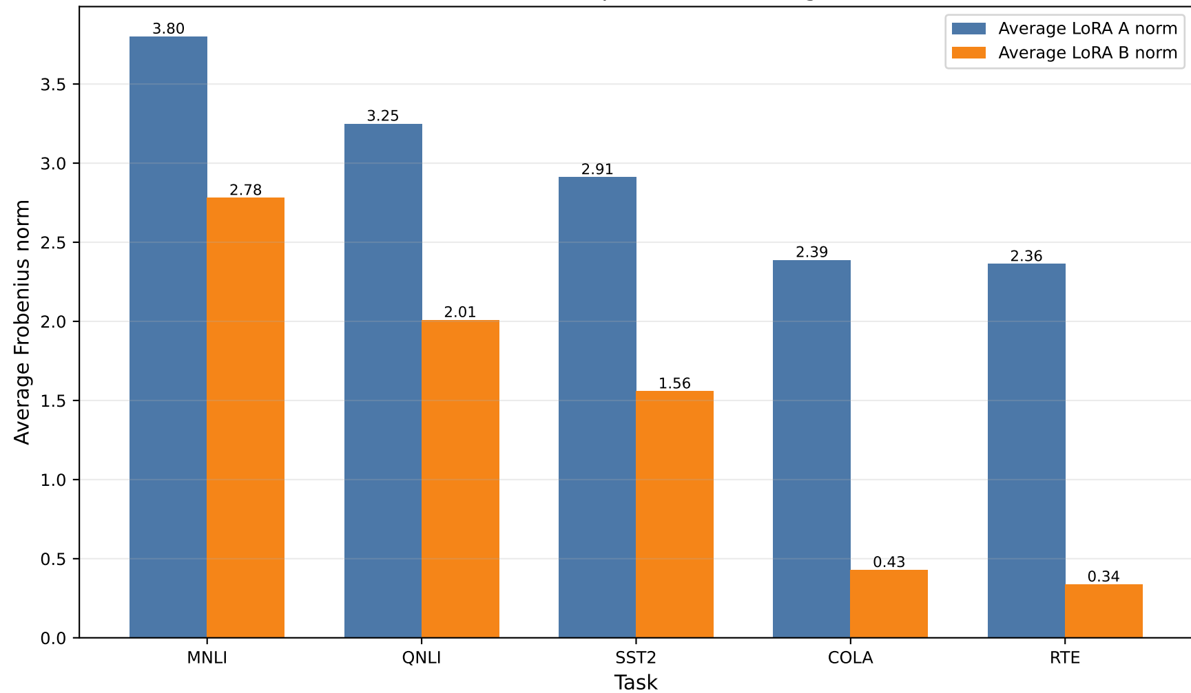
Per-task adapter norm ranking
